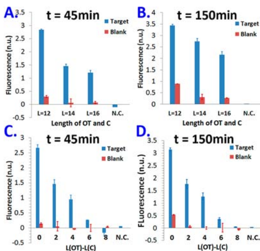
Figure 5. Optimization of the binding-induced DNA strand displacement to minimize the target-independent strand displacement. Streptavidin test solutions contained 5 nM streptavidin, 10 nM OT, 10 nM C, and 20 nM FQ. In the blank, all reagents were the same as streptavidin sample solution, but with no streptavidin added. Effects of simultaneous increases in the length of both OT and C on the performance of the binding-induced strand displacement were monitored at 45 (A) and 150 min (B). Effects of the length difference between OT and C were also monitored at 45 (C) and 150 min (D). The negative control (N.C.) contained only 20 nM FQ in TE-Mg buffer. Error bars represent one standard deviation from duplicated analyses.
