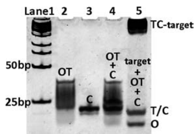
Figure 2. Native PAGE analysis of oligonucleotides from the binding-induced DNA strand displacement. Lane 1, low molecular DNA ladder; lane 2, 2 \mu\text{M} OT; lane 3, 2 \mu\text{M} C; lane 4, from analysis of a mixture containing 2 \mu\text{M} OT and 2 \mu\text{M} C; lane 5, from analysis of a mixture containing 2 \mu\text{M} OT, 2 \mu\text{M} C, and 1 \mu\text{M} streptavidin.
