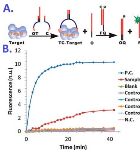
Figure 3. (A) Principle of the binding-induced strand displacement beacon. (B) Evaluation of the binding-induced displacement beacon. The fluorescence intensity was normalized such that 1 normalized unit (n.u.) corresponds to 1 nM O. Control-1 contained the same amount of streptavidin and reagents, except that 500 \mu\text{M} biotin was used to saturate all the binding sites of streptavidin. Control-2 was carried out using the same amount of streptavidin and reagents with the streptavidin sample solution, but without O. Similarly, Control-3 was carried out without competing DNA C, and Control-4 was carried out without OT. In the blank, all reagents were the same as in the streptavidin sample solution, except that there was no streptavidin. Positive control (P.C.), 10 nM O, 20 nM FQ in TE-Mg buffer; negative control (N.C.), only 20 nM FQ in TE-Mg buffer.
